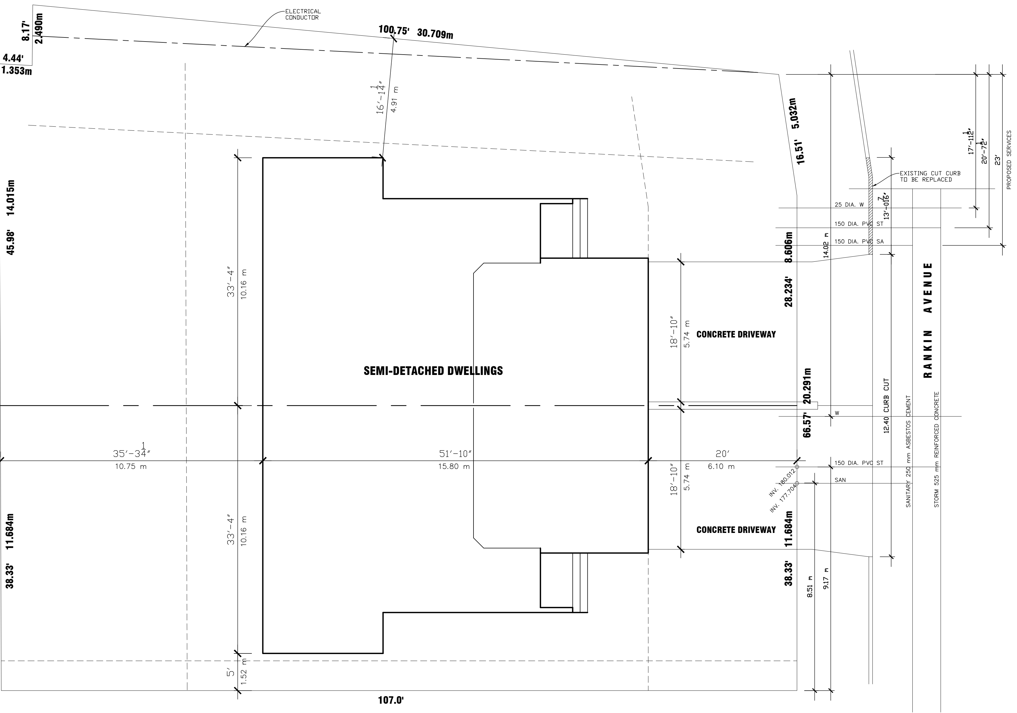
SITE PLAN RANKIN AVENUE - SEMI-DETACHED DWELLINGS
