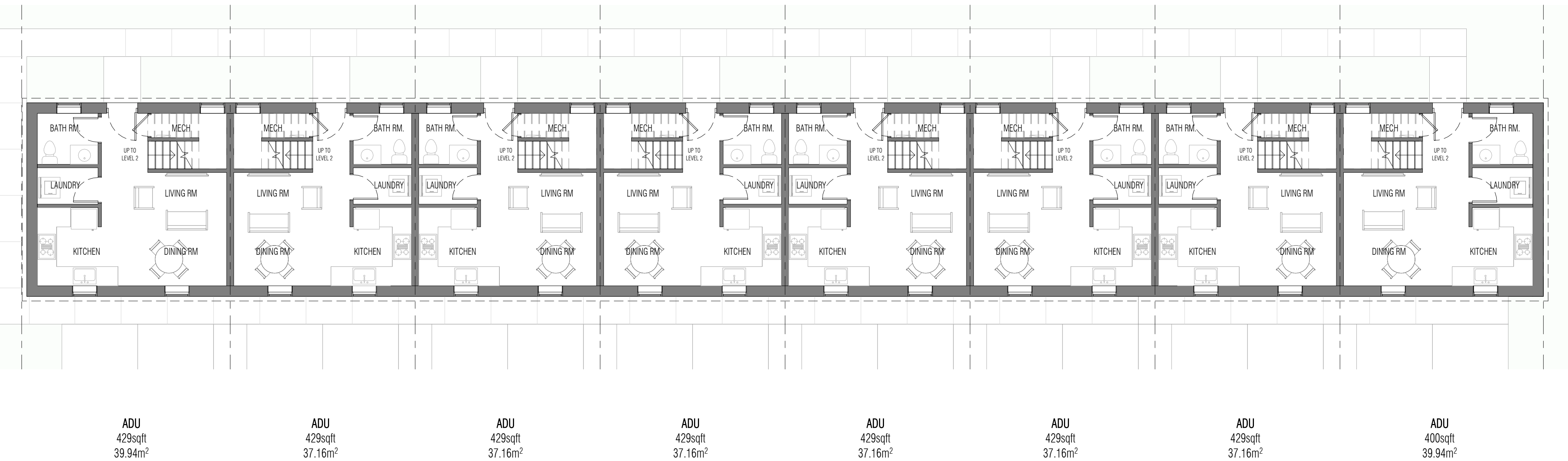
2 FIRST FLOOR PLAN - ADU FP01 1/8" = 1'-0"
