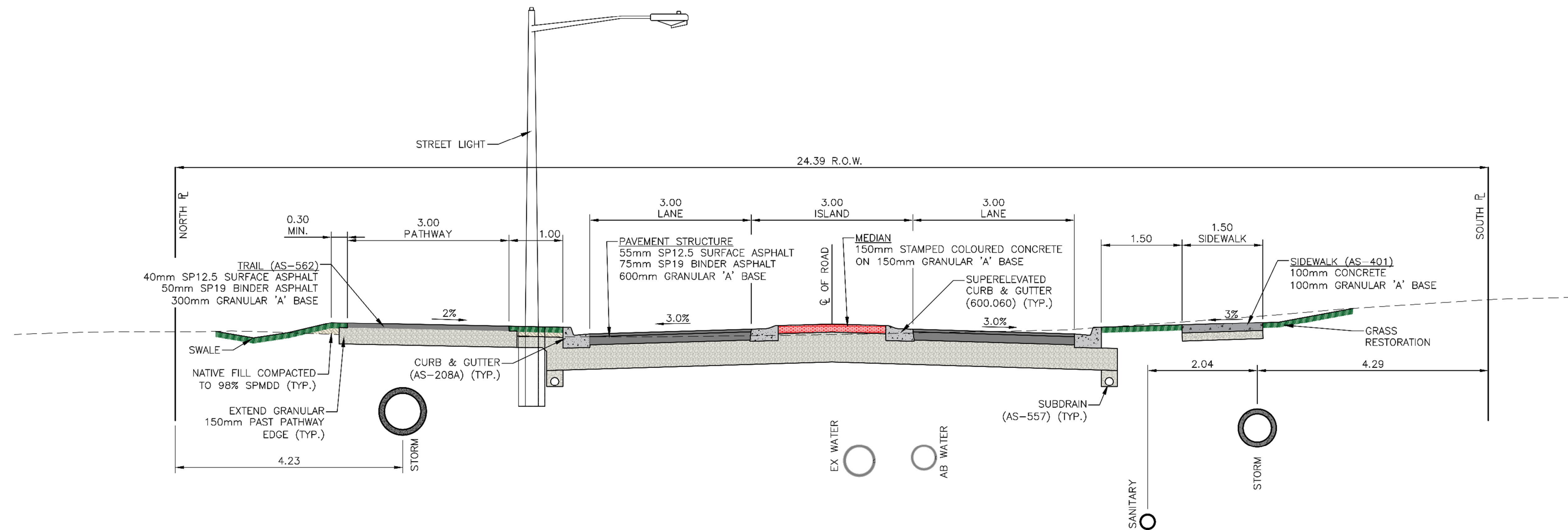
WYANDOTTE STREET STATION 2+240
