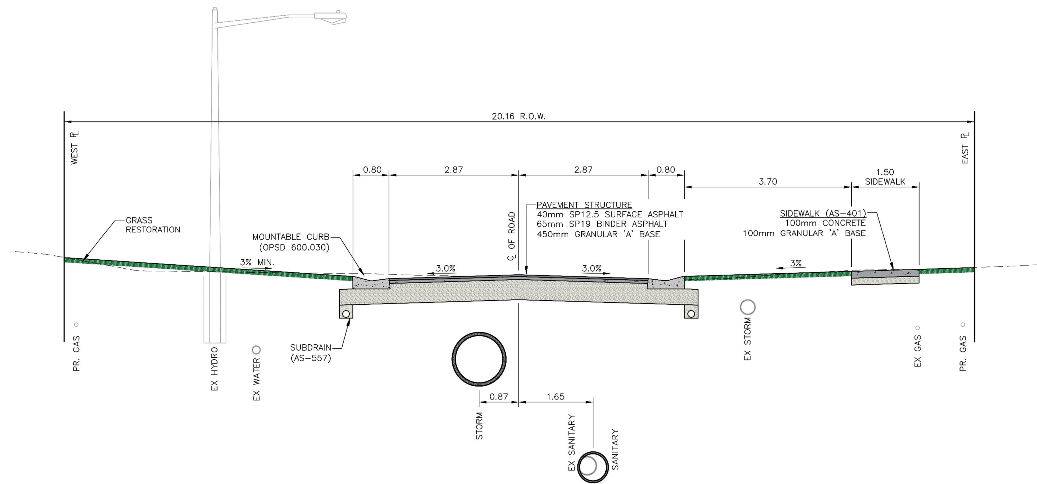
JARVIS AVE WITHOUT BOULEVARD CATCHBASINS
