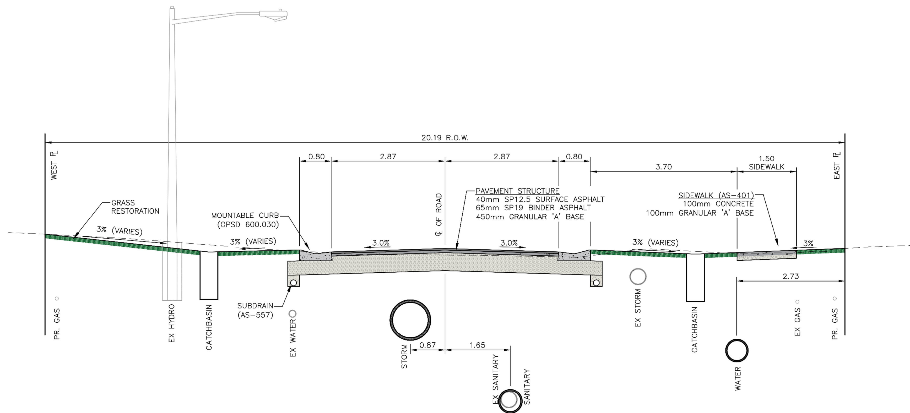
JARVIS AVE WITH BOULEVARD CATCHBASINS
