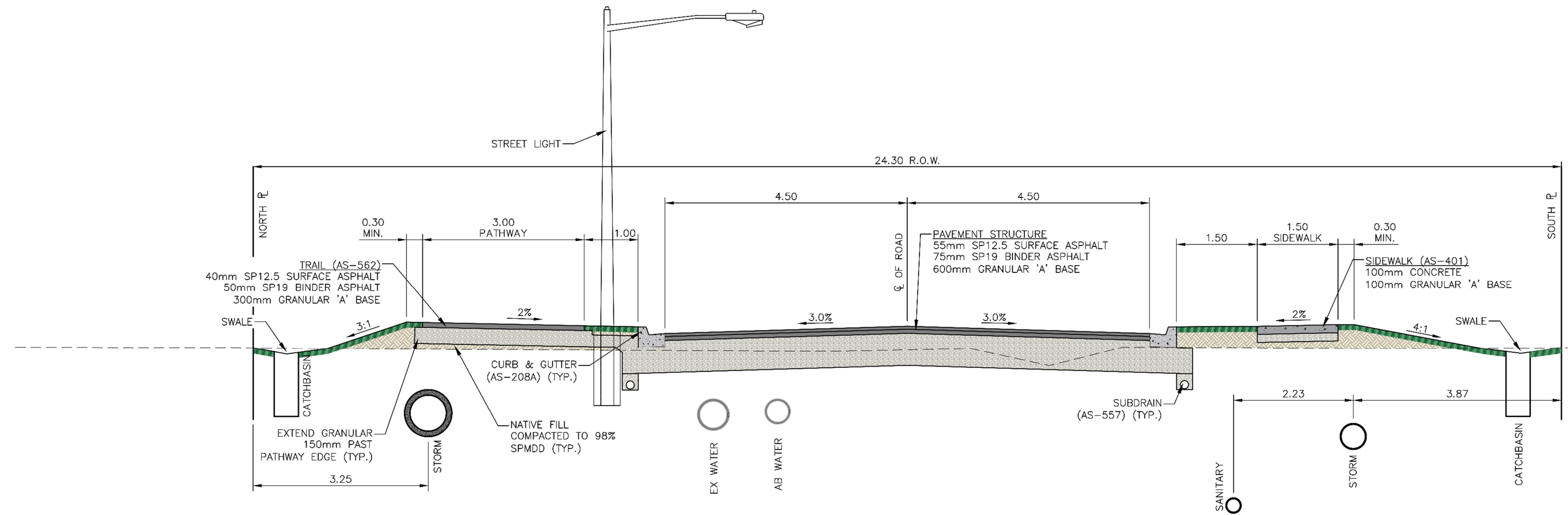
WYANDOTTE STREET STATION 1+150
