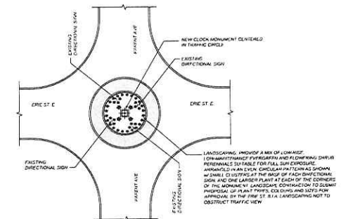
PLAN OF ERIE-PARENT ROUNDBABOUT SCALE: 1/4" = 1'-0"
