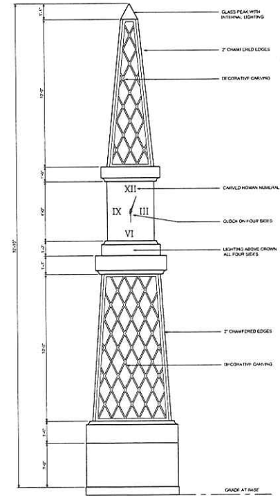
CLOCK MONUMENT ELEVATION SCALE: 1/4" = 1'-0"
