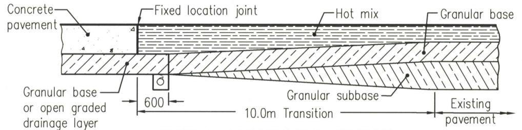
TYPE A: LONGITUDINAL SECTION CONCRETE PAVEMENT TO HOT MIX PAVEMENT WITH GRANULAR BASE
