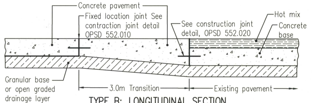
TYPE B: LONGITUDINAL SECTION CONCRETE PAVEMENT TO COMPOSITE PAVEMENT
