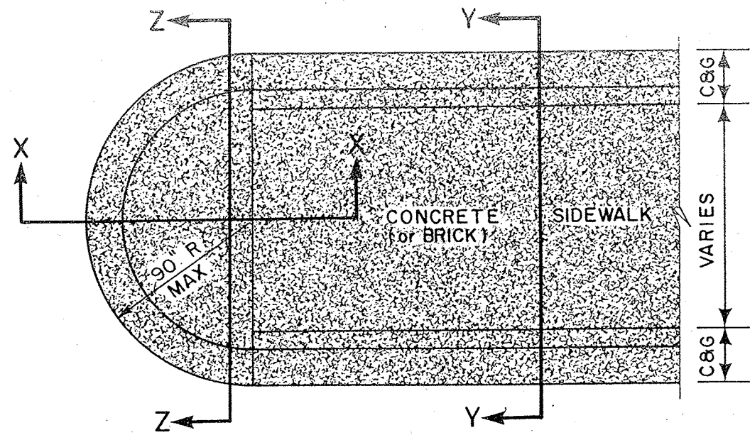
OVER 42" RADIUS END TREATMENT
