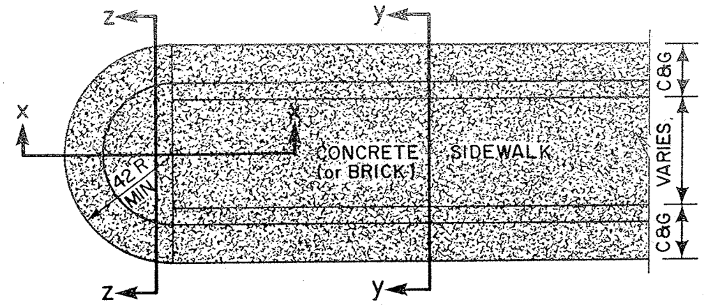
42" RADIUS END TREATMENT
